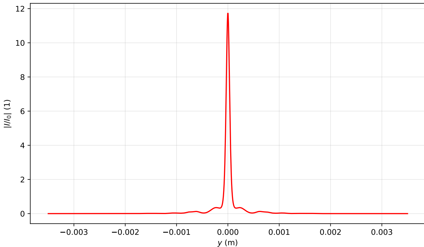
Intensity profile I(x=0, y, z=1.433)/I_0 , P_{in}=6.5P_{cr} , artificial time
